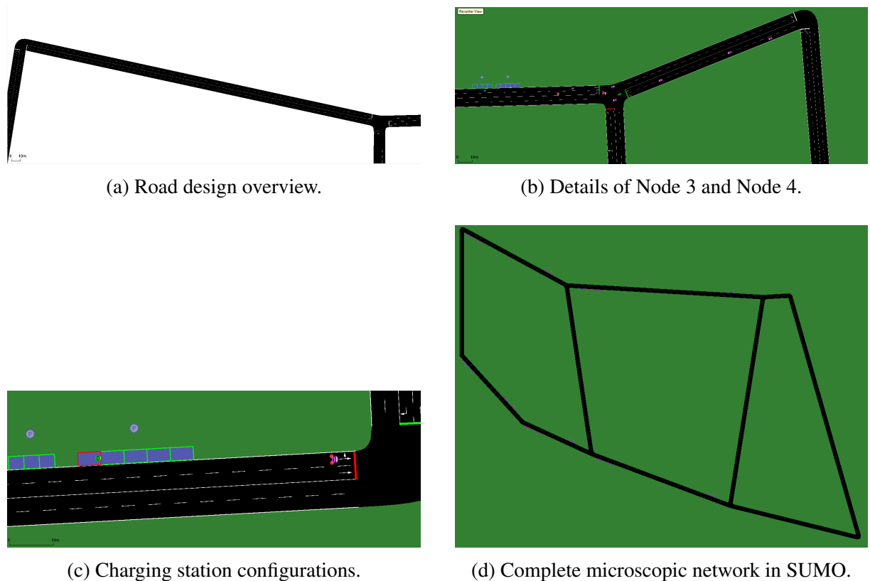
Figure 3.3: Custom microscopic road network in SUMO netedit : (a) design, (b) Nodes 3-4, (c) charging slots, and (d) complete network.
